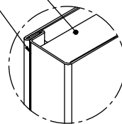
STANDARD LOCKSEAM EDGE & OPTIONAL FLUSH CAP DETAIL
