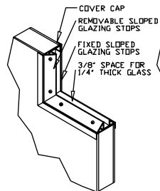
SPECIAL SLOPED GLAZING KIT
