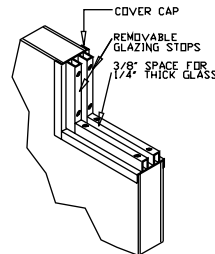
STANDARD GLAZING KIT
