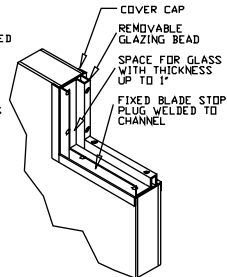
THICK GLASS GLAZING KIT
