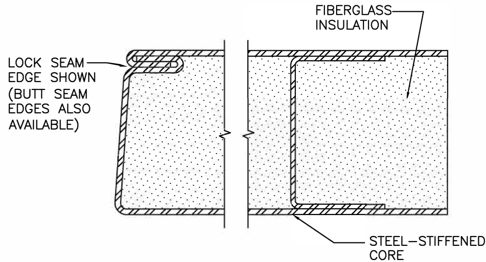
DETAIL "C" 1"-0" = 1'-0"
