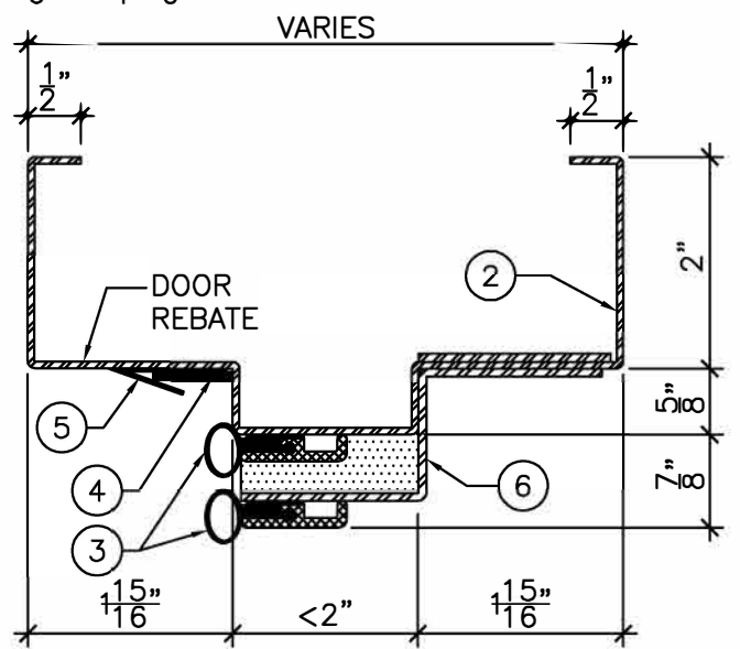
DETAIL "A" - LESS THAN 2" SOFFIT \frac{6}{6}'' = 1'-0''
