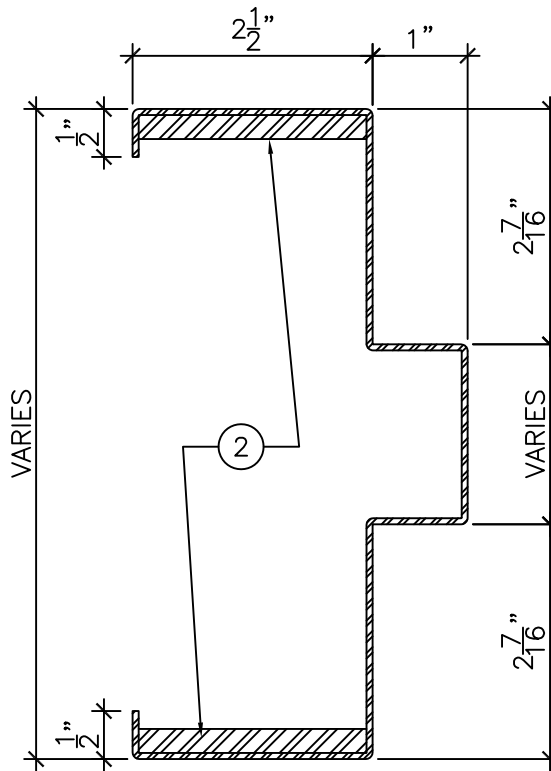
DETAIL "A" 6" = 1'-0"
