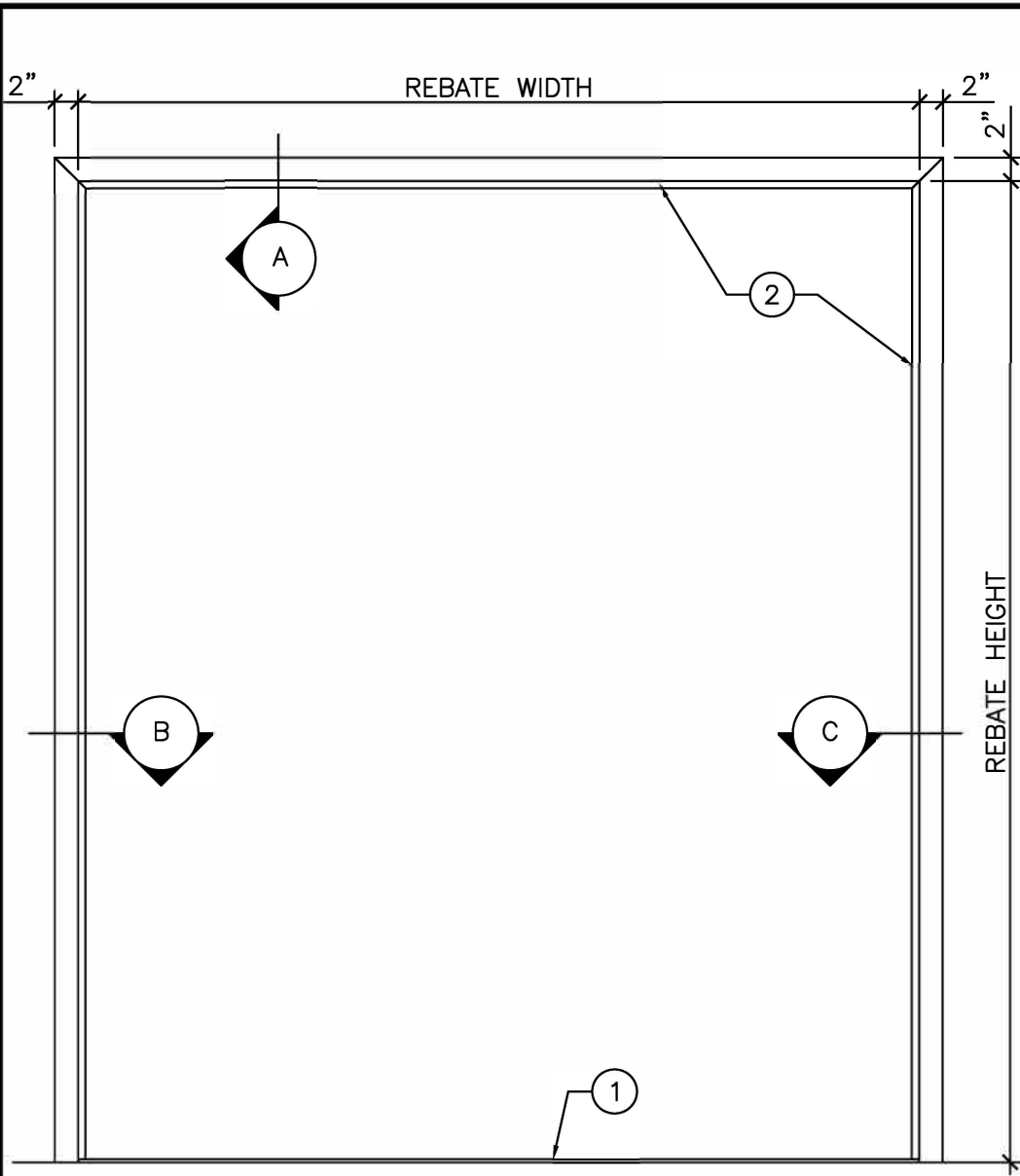
ELEVATION 3/4" = 1'-0"
