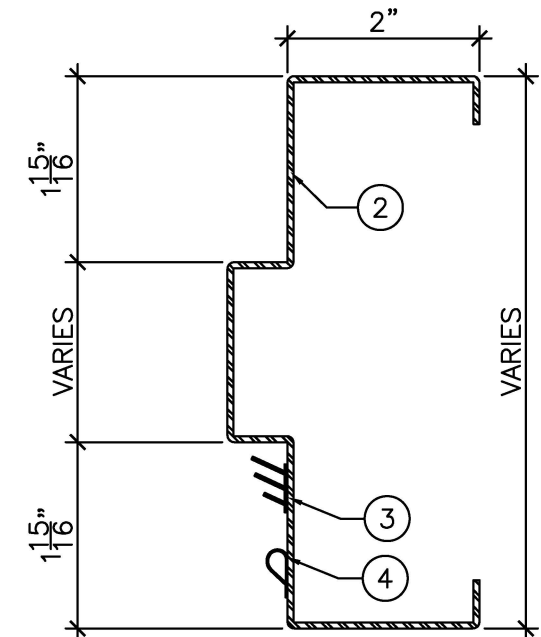
DETAIL "C" 6" = 1'-0"
