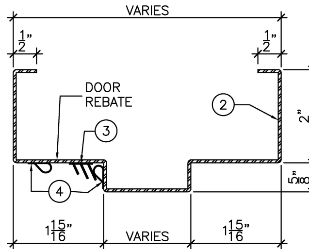
DETAIL "A" 6" = 1'-0"
