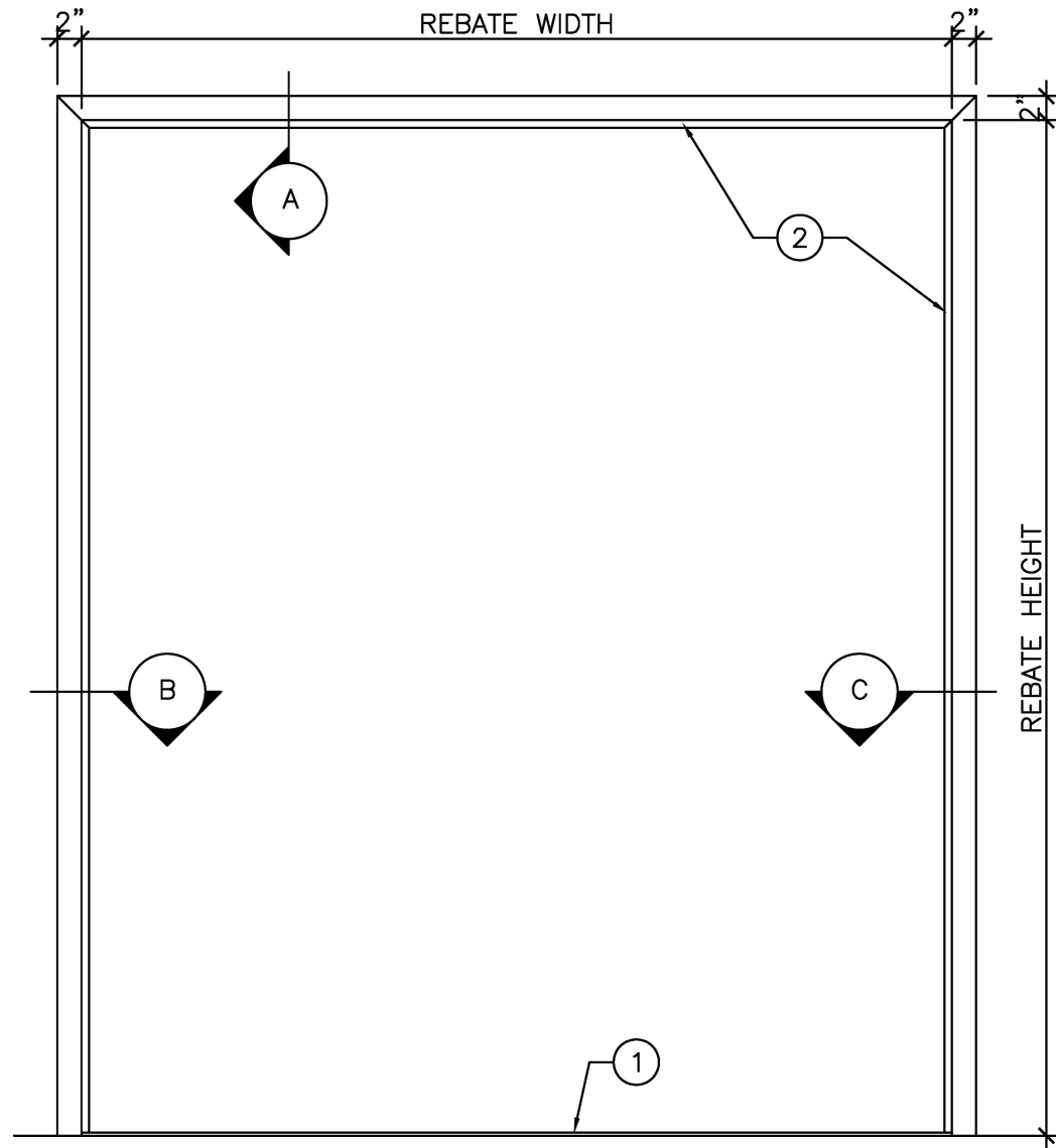
ELEVATION 3/4" = 1'-0"
