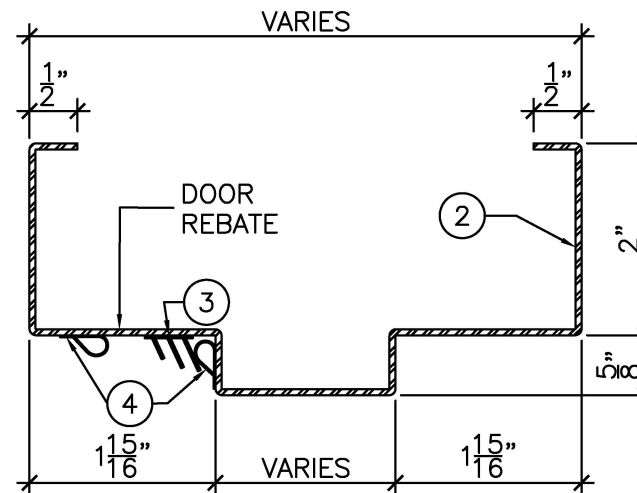
DETAIL "A" 6" = 1'-0"
