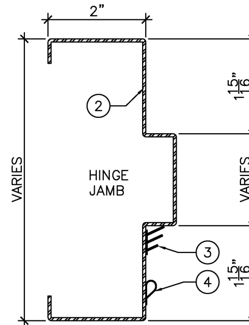
DETAIL "B" 6" = 1'-0"
