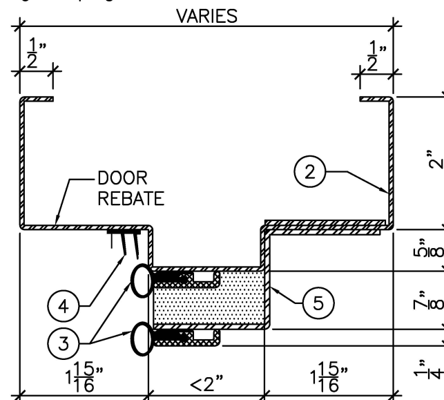
DETAIL "A" - LESS THAN 2" SOFFIT
