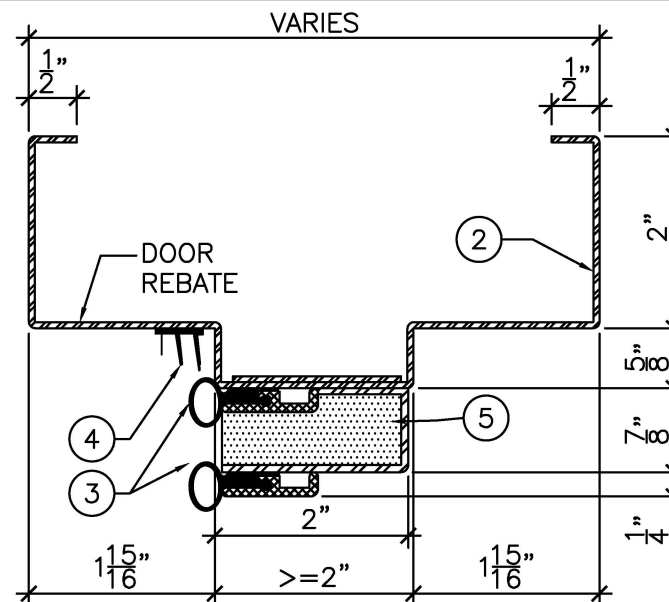
DETAIL "A" - 2" SOFFIT OR MORE
