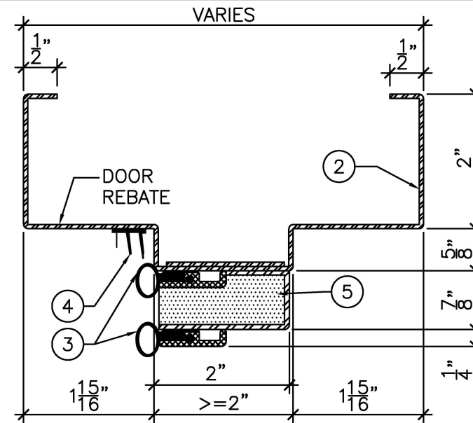
DETAIL "A" - 2" SOFFIT OR MORE \frac{6"}{6"} = 1'-0"
