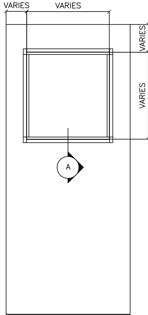
SECTION "A" 3/4" = 1'-0"
