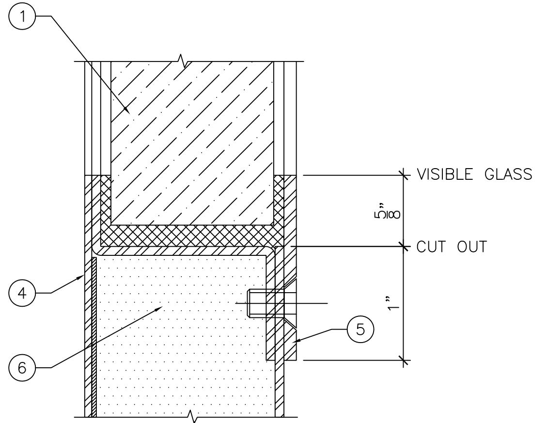
SECTION "A" 1'-0" = 1'-0"
