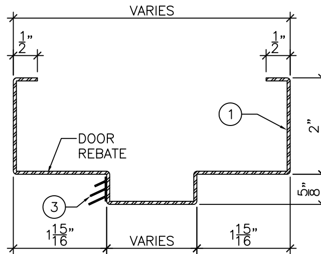
DETAIL "A" 6" = 1'-0"
