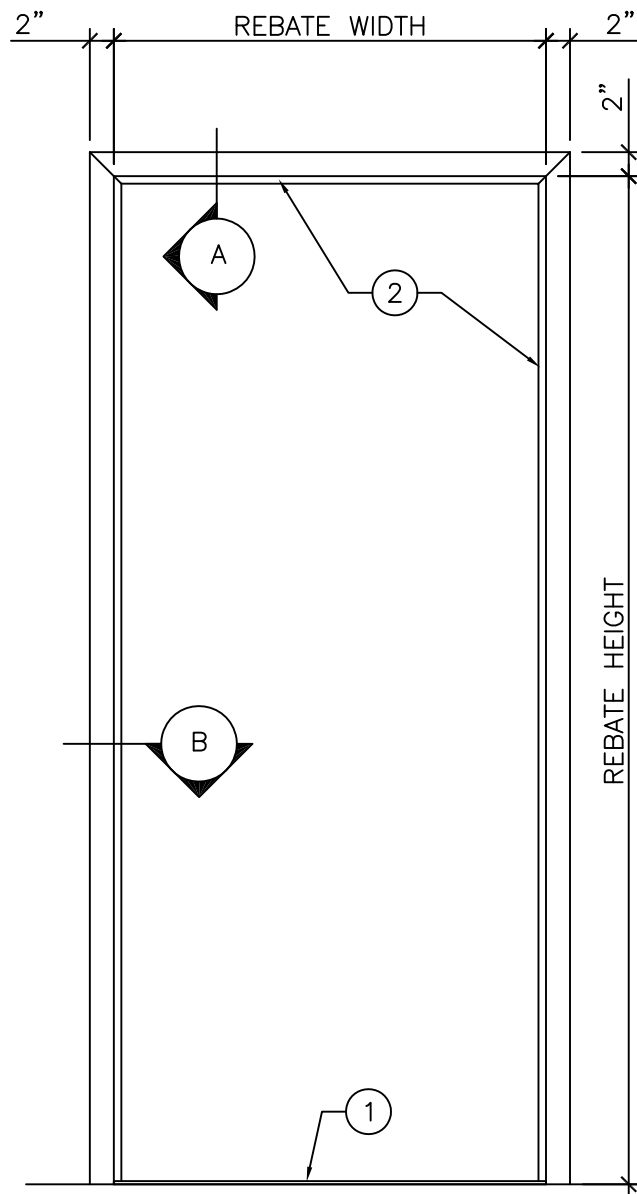
ELEVATION 3/4" = 1'-0"
