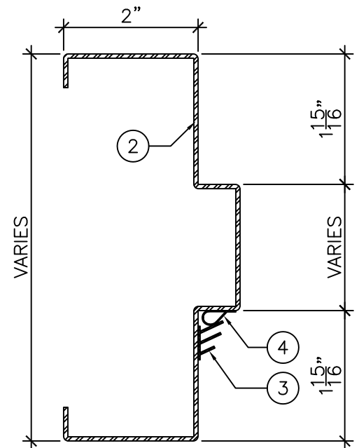
DETAIL "B" 6" = 1'-0"
