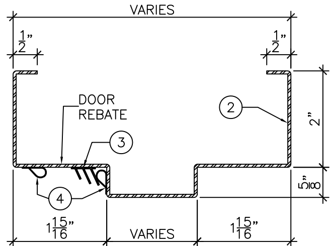
DETAIL "A" 6" = 1'-0"
