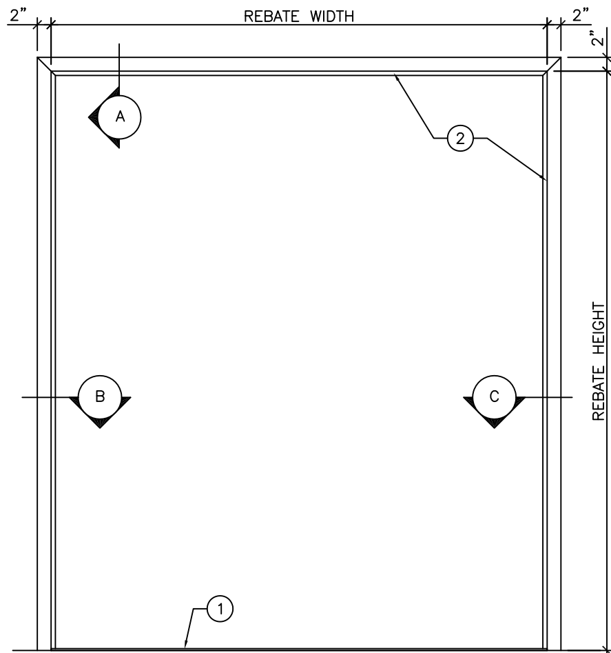
ELEVATION 5/8" = 1'-0"
