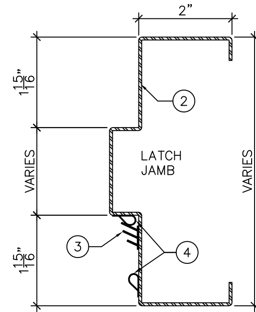
DETAIL "C" 6" = 1'-0"
