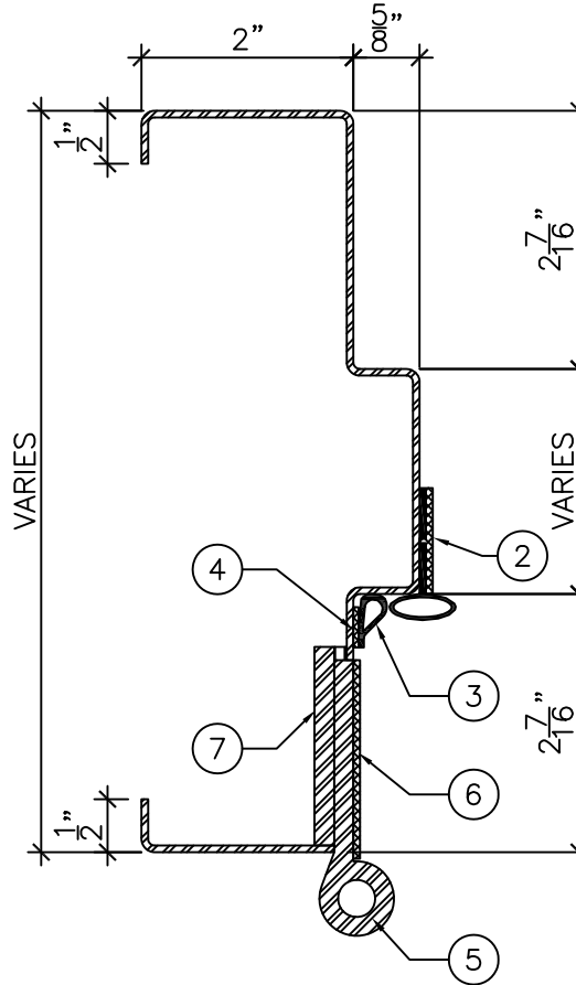
DETAIL "A" 6" = 1'-0"
