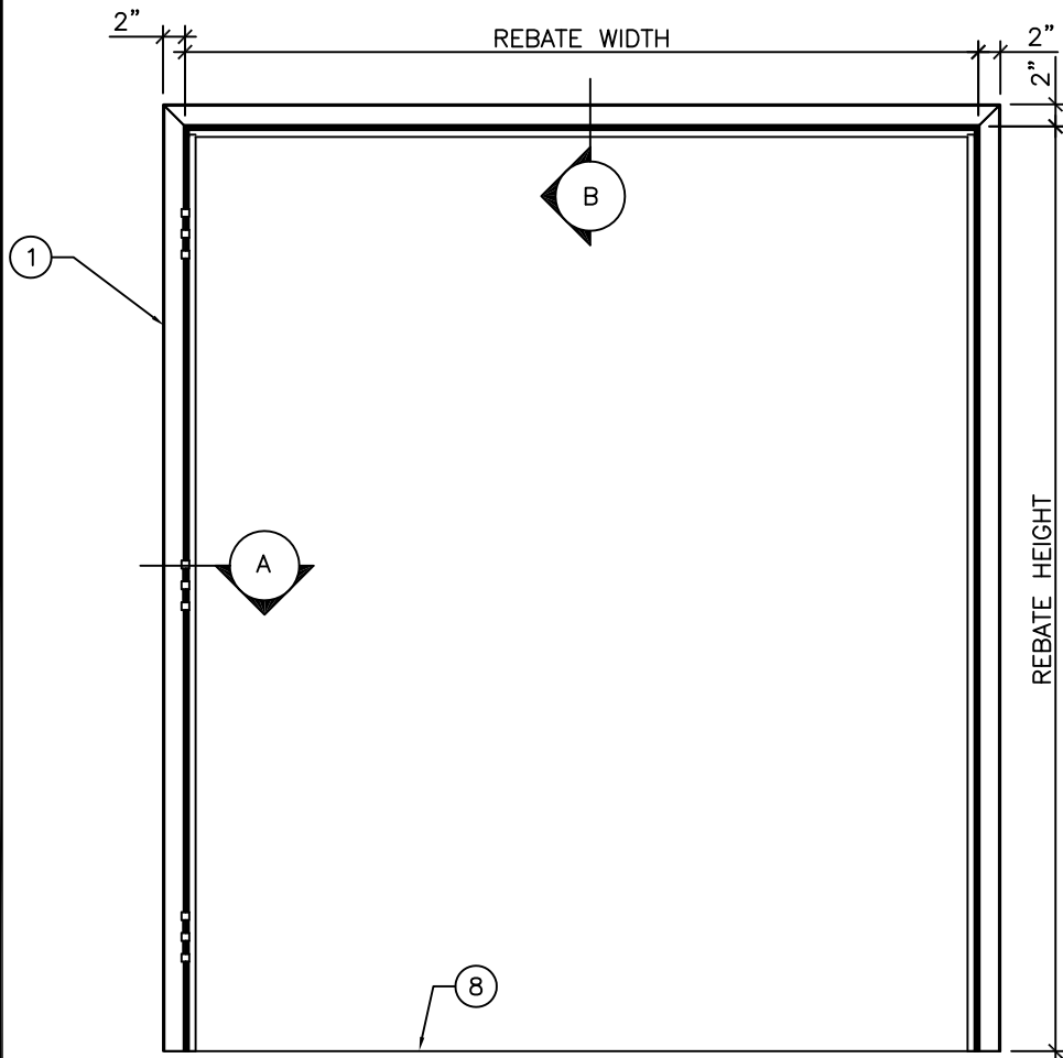
ELEVATION 5/8" = 1'-0"
