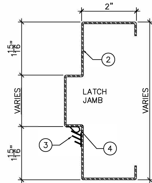
DETAIL "C" 6" = 1'-0"
