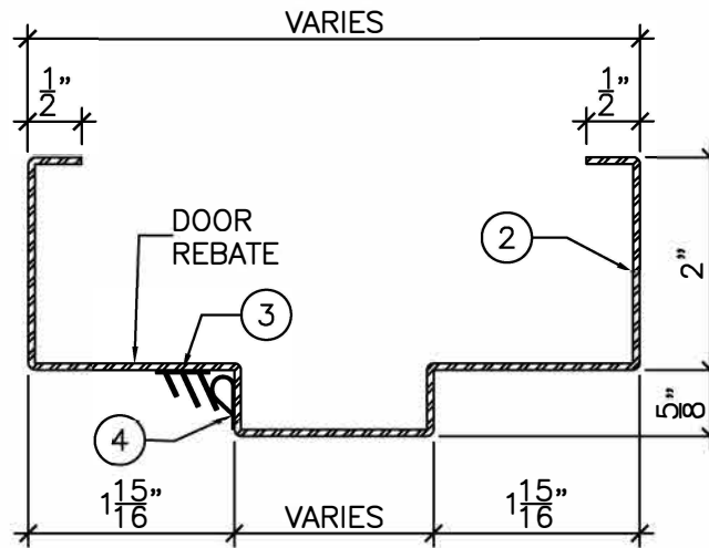
DETAIL "A" 6" = 1'-0"
