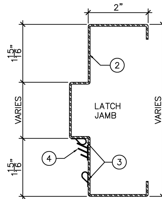
DETAIL "C"
