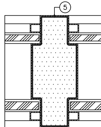
DETAIL "B" 3"-0" = 1'-0"
