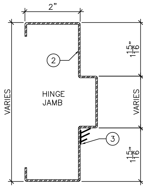
DETAIL "B" 6" = 1'-0"
