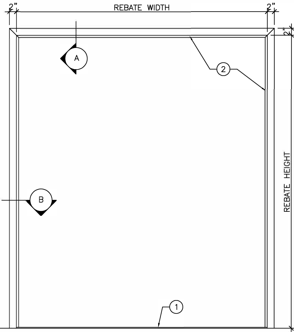
ELEVATION 3/4" = 1'-0"
