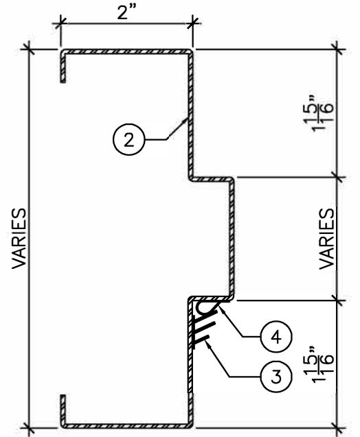
DETAIL "B" 6" = 1'-0"
