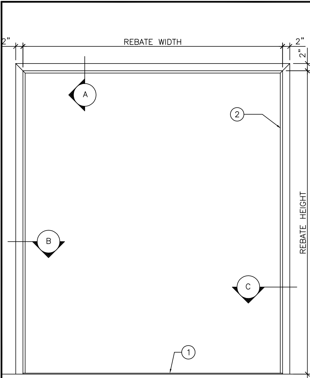
ELEVATION 3/4" = 1'-0"
