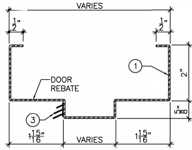
DETAIL "A" 6" = 1'-0"
