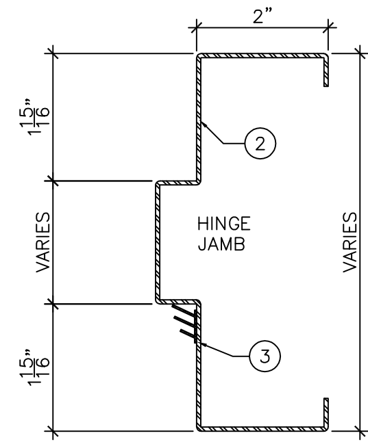
DETAIL "C" 6" = 1'-0"
