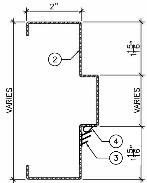
DETAIL "B" 6" = 1'-0"
