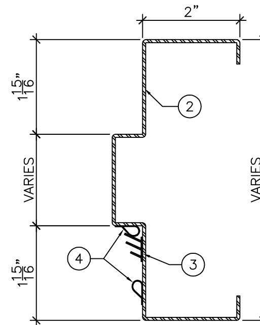
DETAIL "C" 6" = 1'-0"
