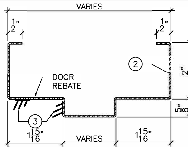
DETAIL "A" 6" = 1'-0"
