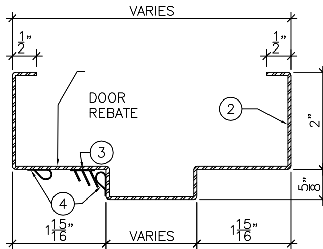
DETAIL "A" 6" = 1'-0"
