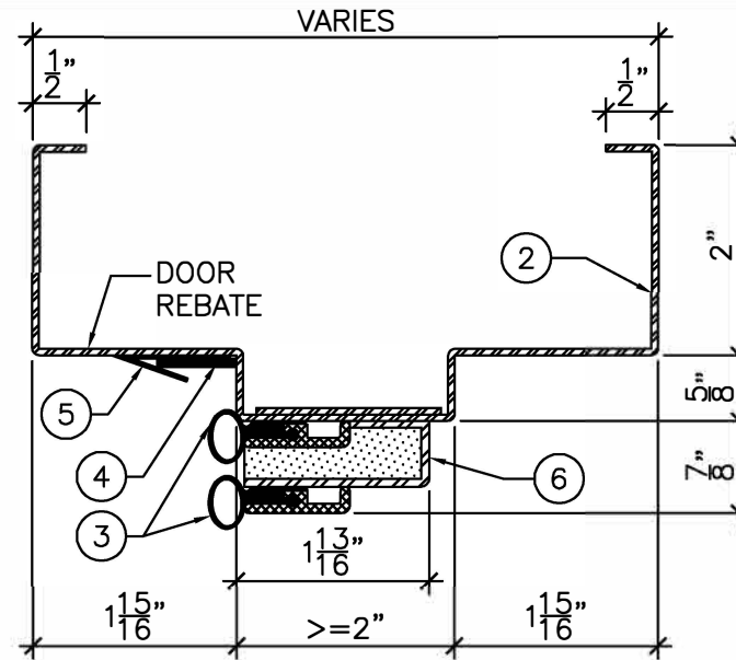
DETAIL "A" - 2" SOFFIT OR MORE \frac{6}{8}'' = 1'-0''
