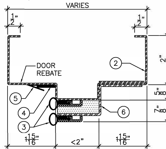
DETAIL "A" - LESS THAN 2" SOFFIT \frac{6}{8}'' = 1'-0''
