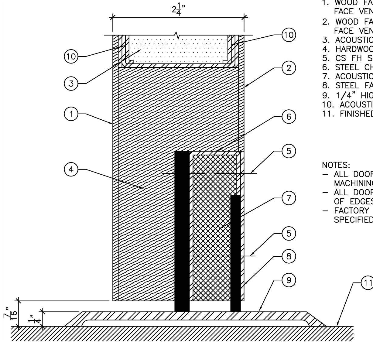
BOTTOM DETAIL "A" 1'-0" = 1'-0"
