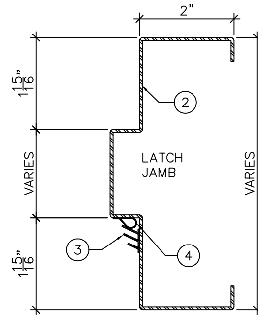
DETAIL "C"
