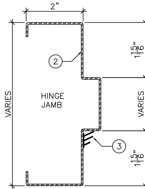
DETAIL "B"
