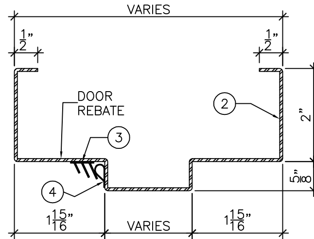
DETAIL "A"
