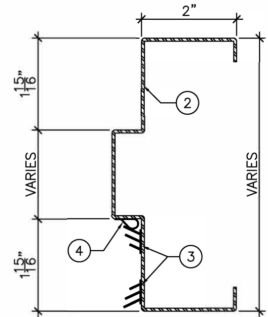
DETAIL "C" 6" = 1'-0"
