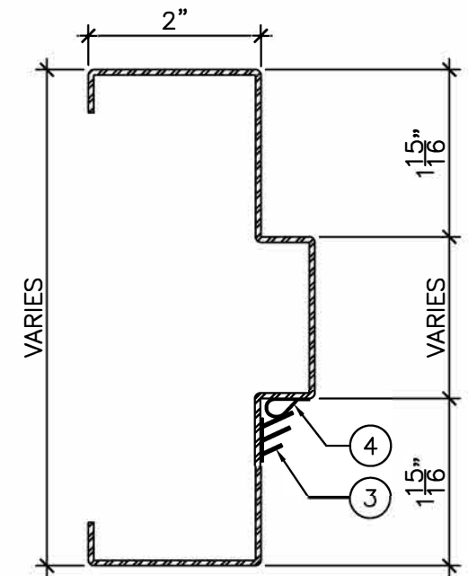
DETAIL "B" 6" = 1'-0"
