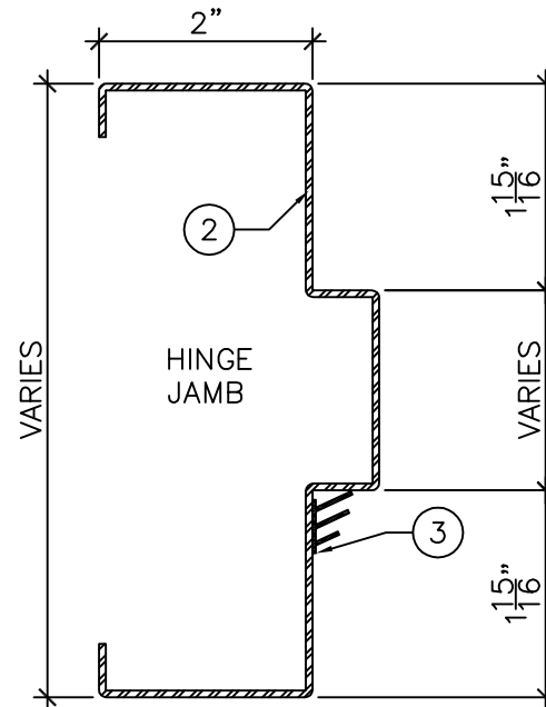
DETAIL "B" 6" = 1'-0"
