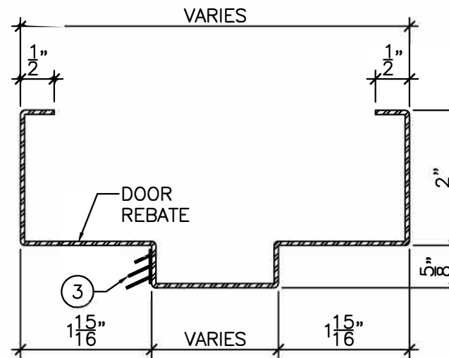
DETAIL "A" 6" = 1'-0"
