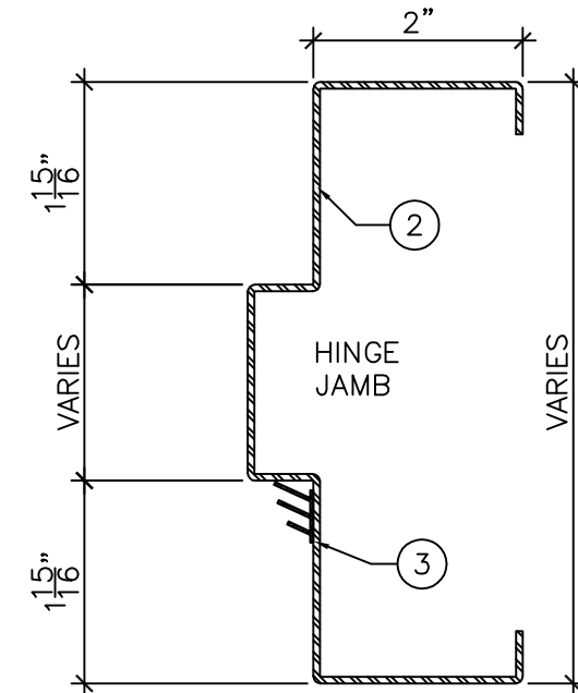
DETAIL "C" 6" = 1'-0"
