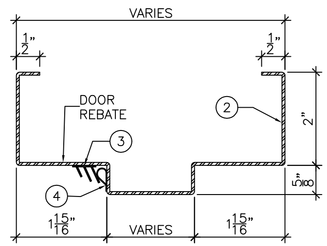
DETAIL "A" 6" = 1'-0"
