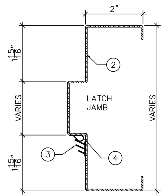
DETAIL "C" 6" = 1'-0"
