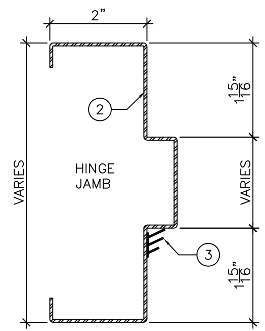
DETAIL "B" 6" = 1'-0"
