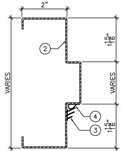
DETAIL "B" 6" = 1'-0"
