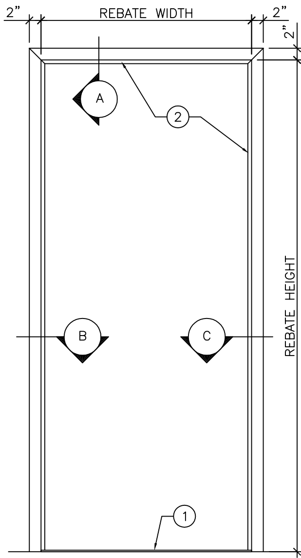
ELEVATION 3/4" = 1'-0"
