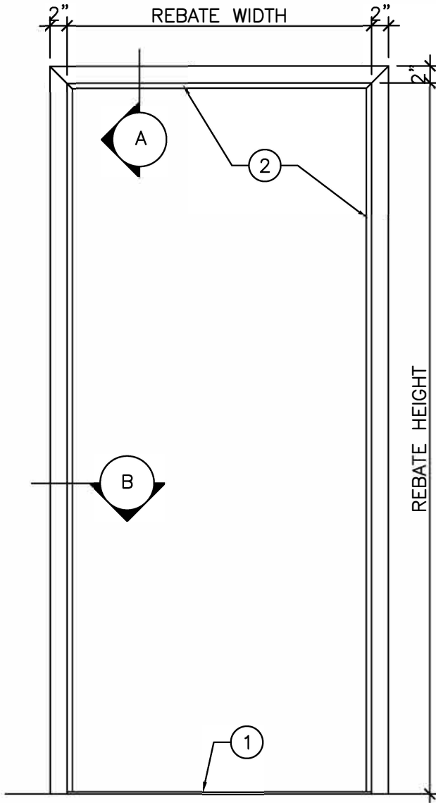
ELEVATION 3/4" = 1'-0"
