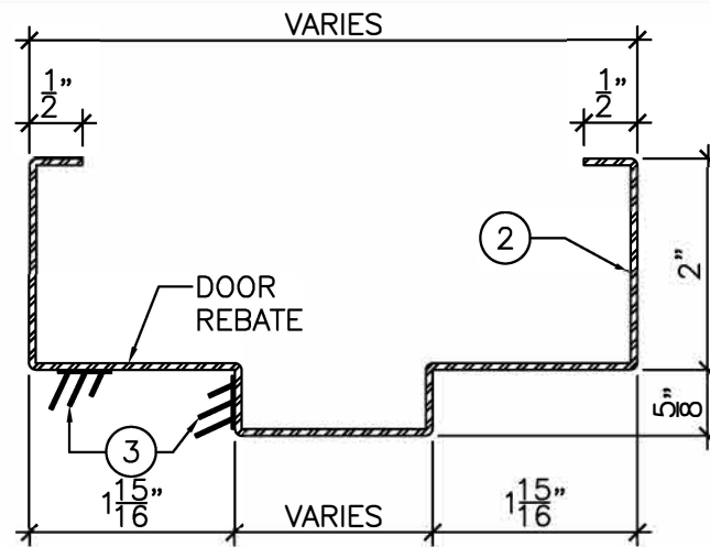
DETAIL "A" 6" = 1'-0"
