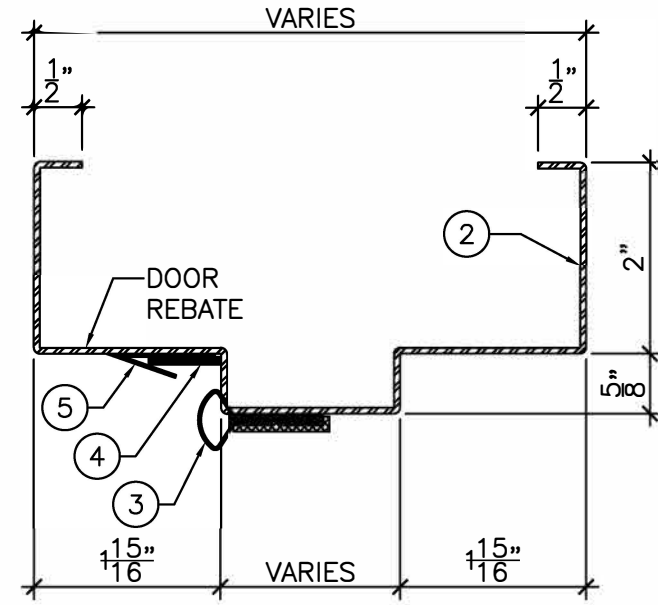
DETAIL "A" 6" = 1'-0"
