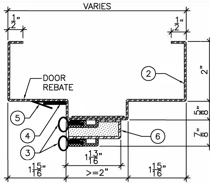
DETAIL "A" \frac{6}{2}'' = 1'-0''
