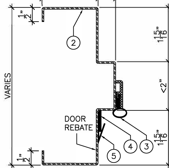
DETAIL "B" \frac{6}{2}'' = 1'-0''
