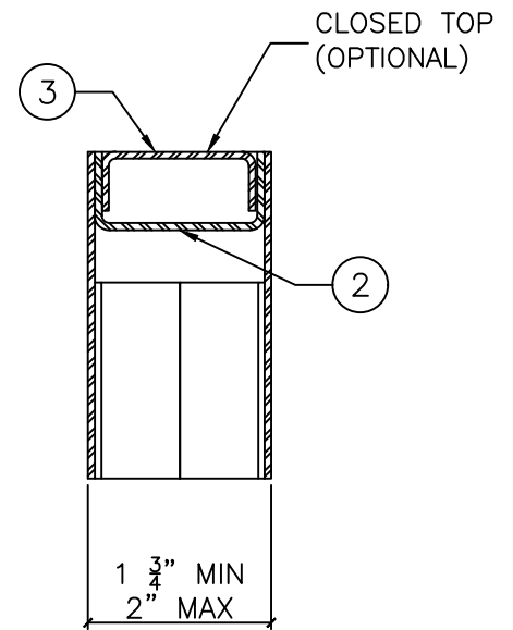
DETAIL "A" 6"-0" = 1'-0"
