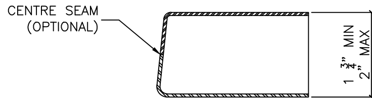
DETAIL "B" 6"-0" = 1'-0"
