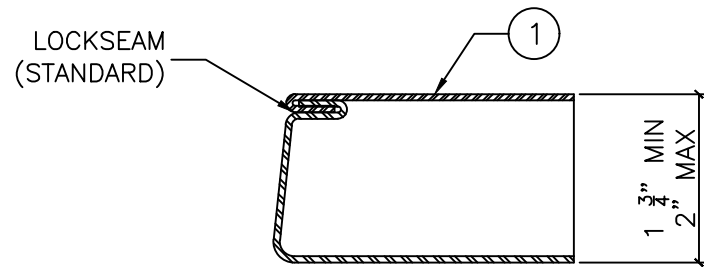
DETAIL "B" 6"-0" = 1'-0"
