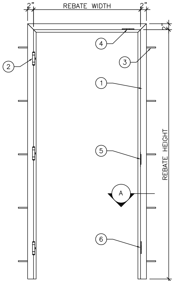
ELEVATION 3/4" = 1'-0"
